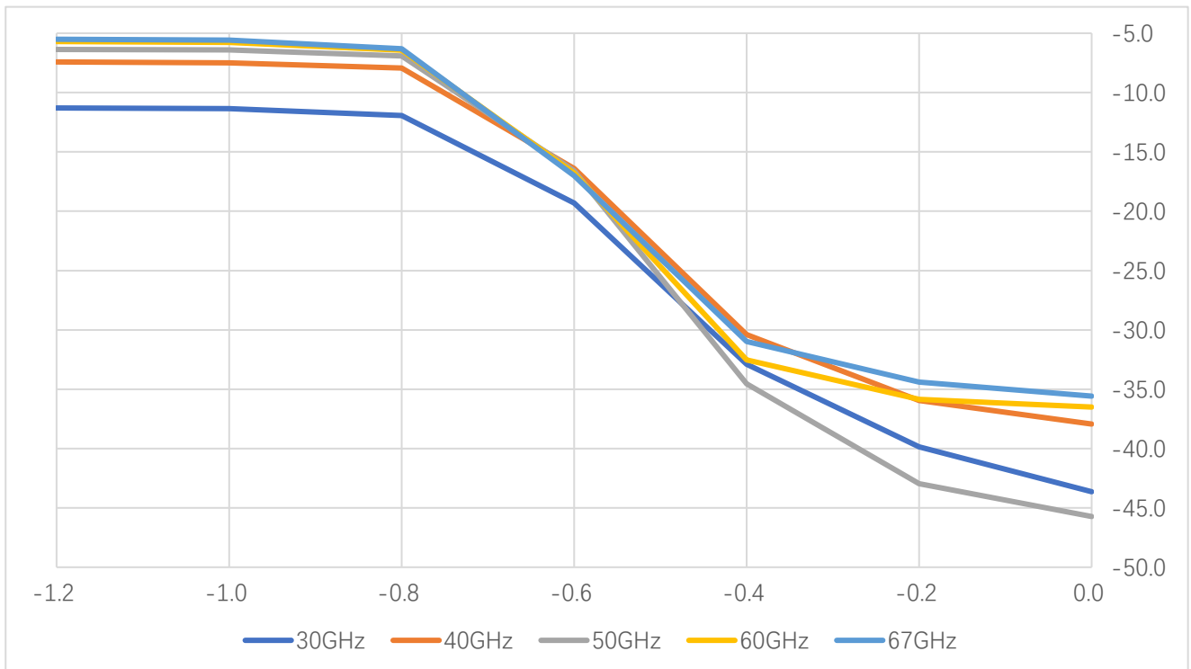
Attenuation Range vs Frequency
