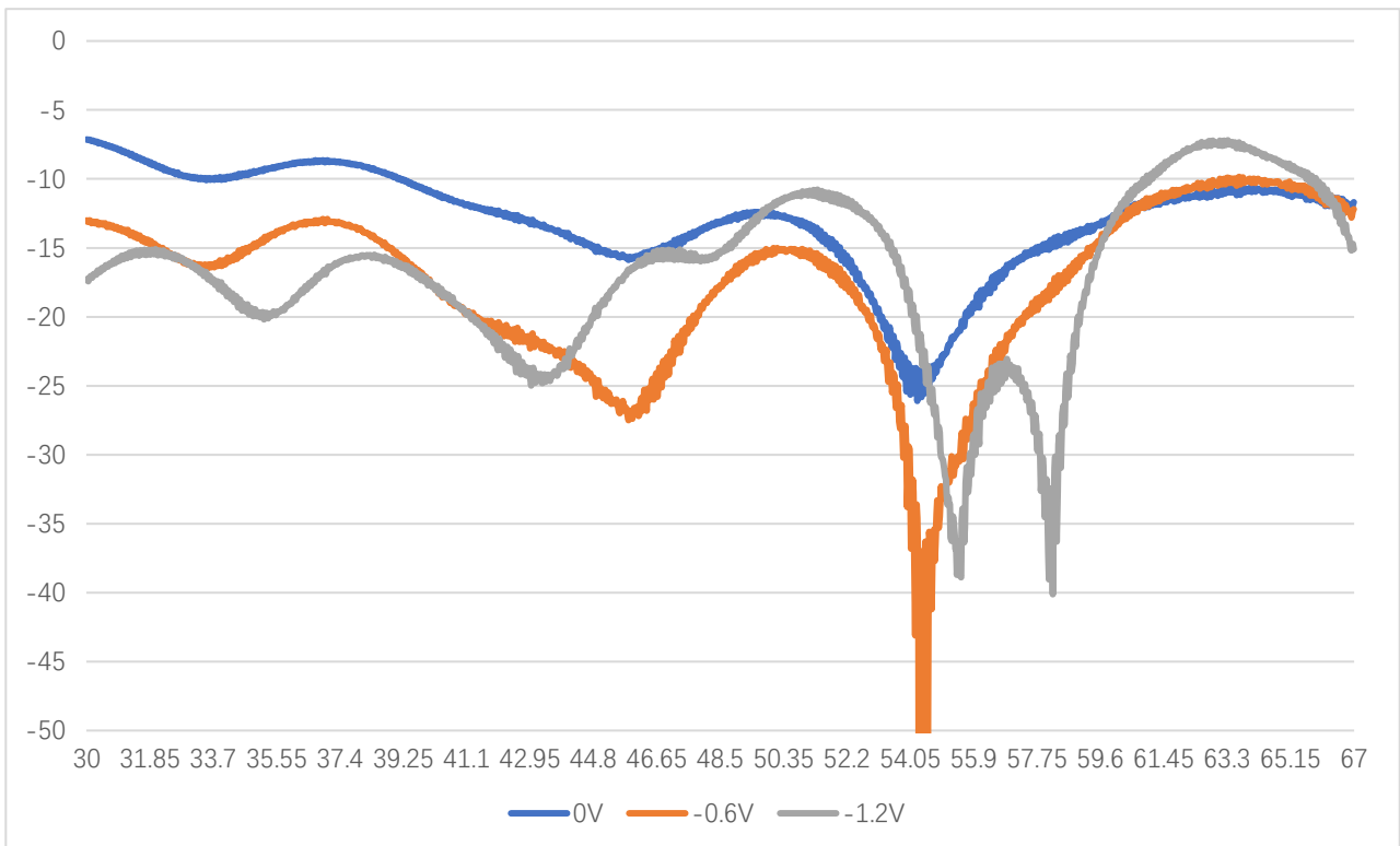
S22 vs Frequency
