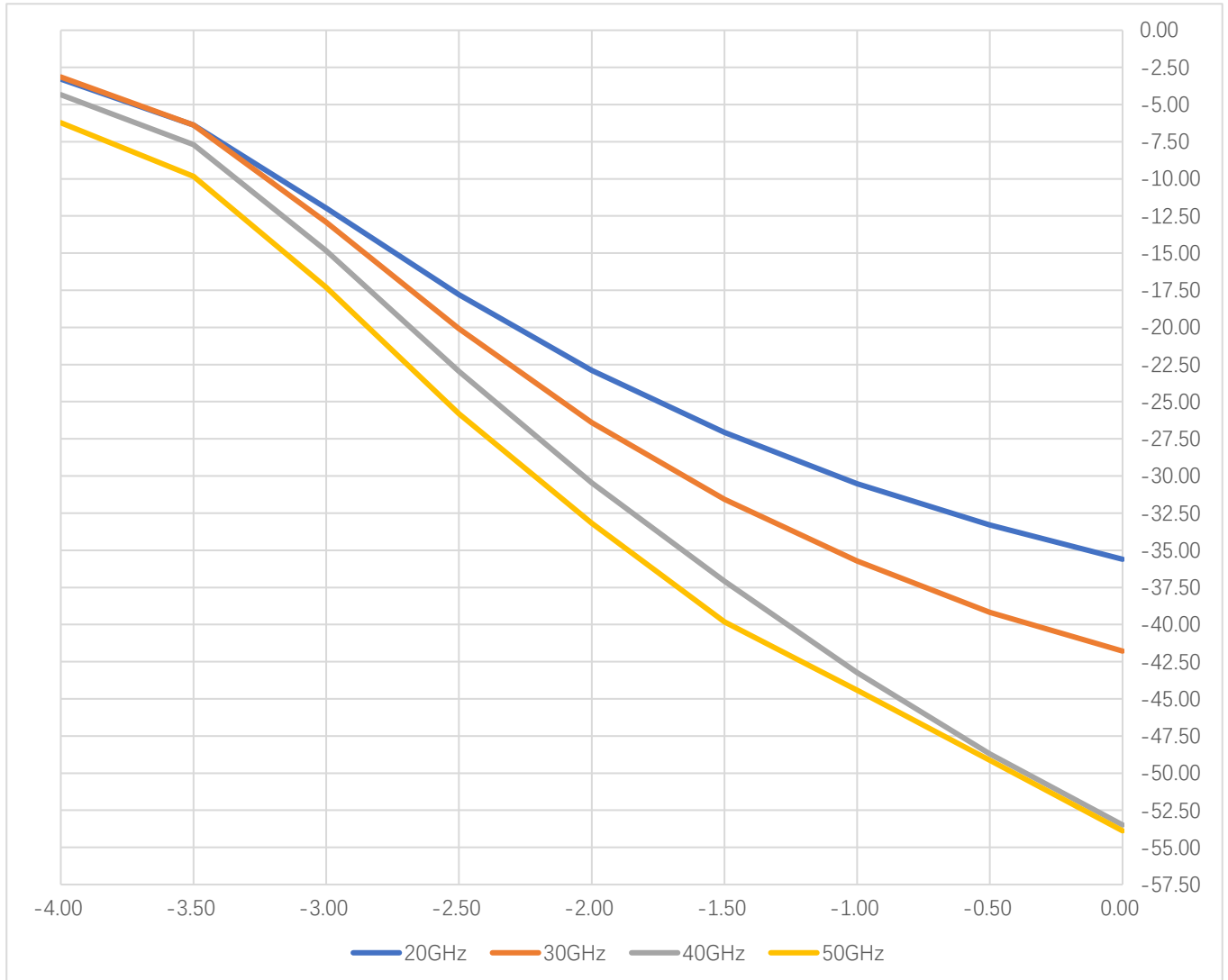
Attenuation vs Voltage at 20/30/40GHz
