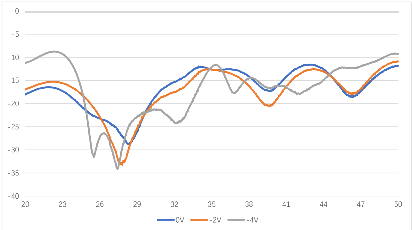
S11 Return Loss at 0/-2/-4V Control Voltage
