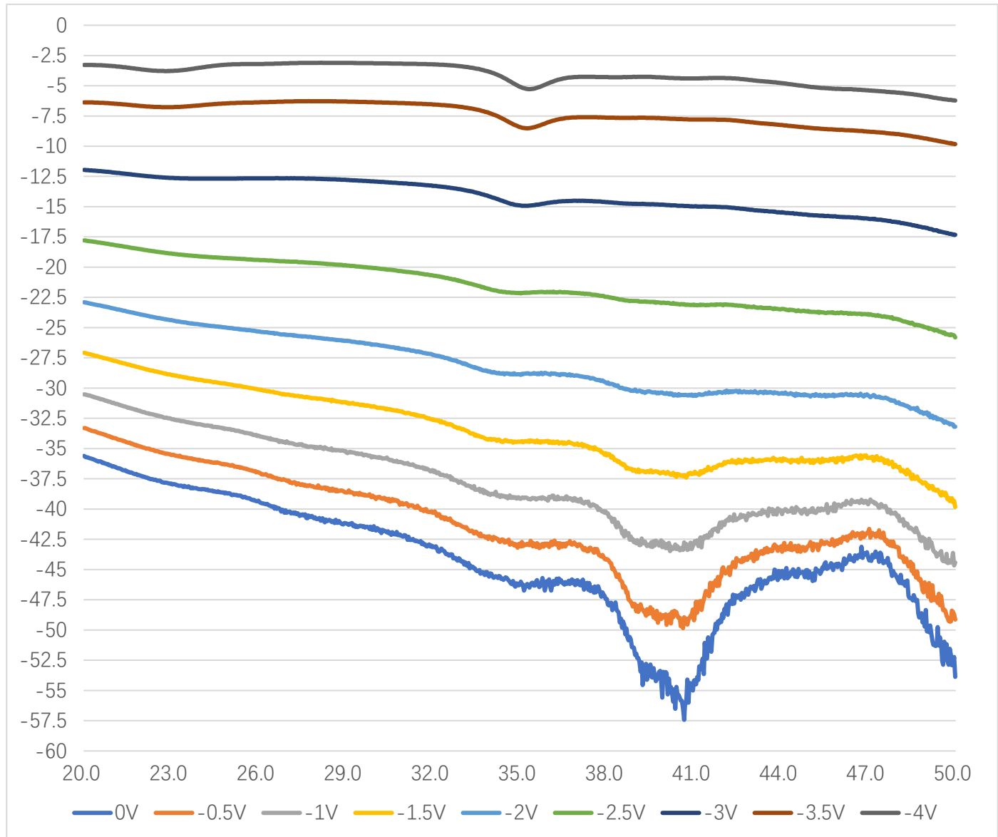
Attenuation vs Voltage Control
