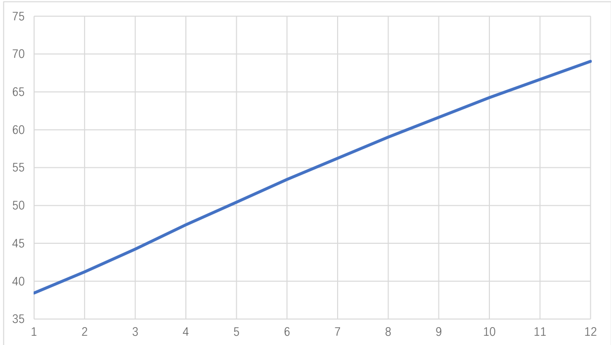
Output Frequency vs Tuning Voltage
