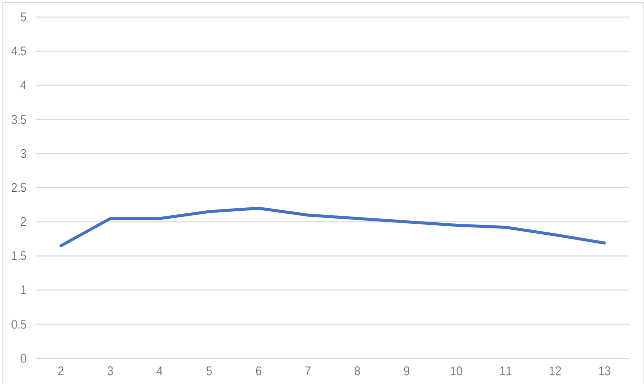
Sensitivity GHz/V vs Tuning Voltage
