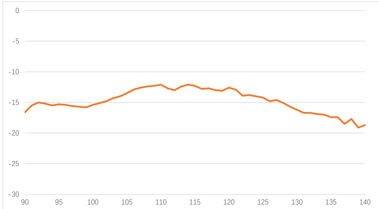
Conversion Loss vs Frequency at Pin=+18dBm
