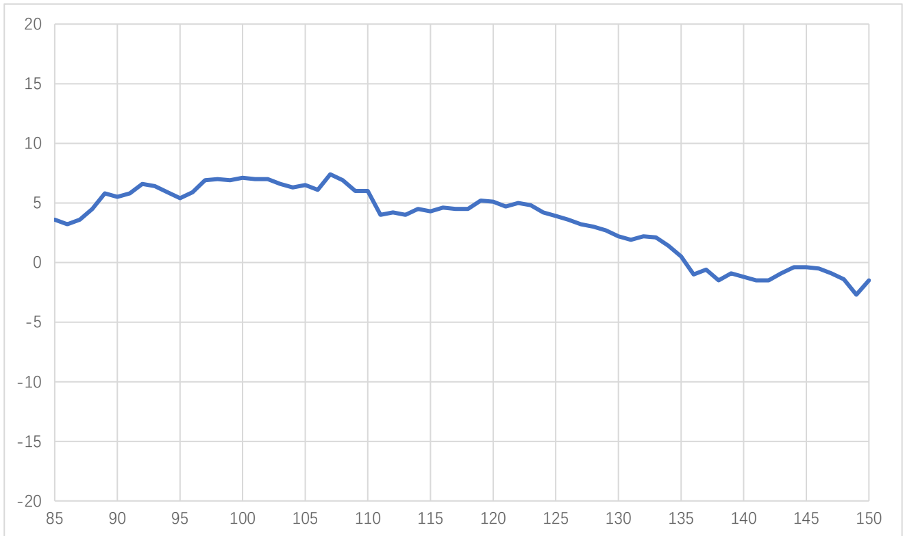
Pout vs Frequency AT-AM4-4580C-15L used as Driver
