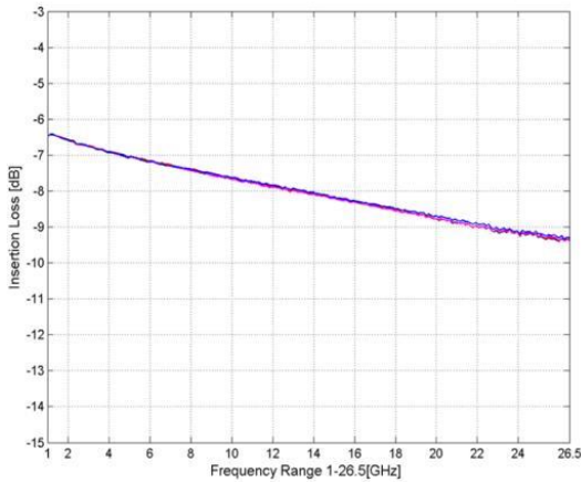
Figure 3: Insertion Loss
