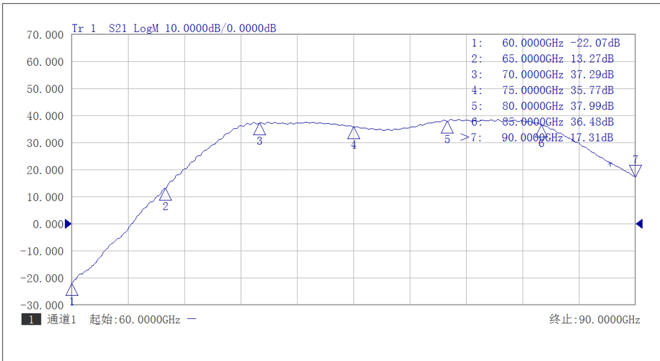
Gain vs Frequency, 60-90GHz
