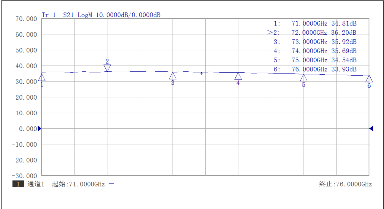
Gain vs Frequency, 71-76GHz
