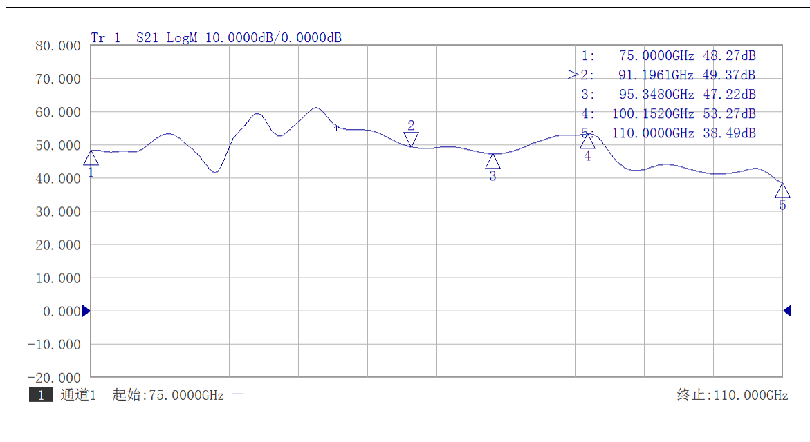
Gain vs Frequency 75-110GHz
