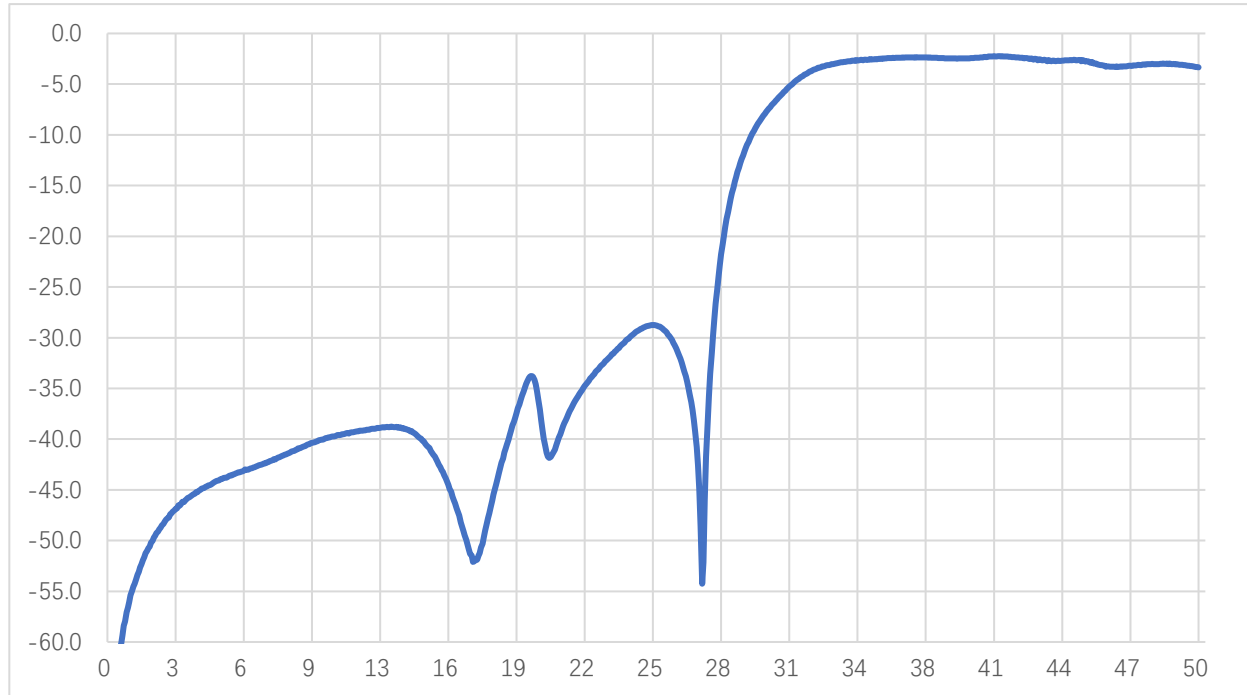
S21 vs Frequency/GHz
