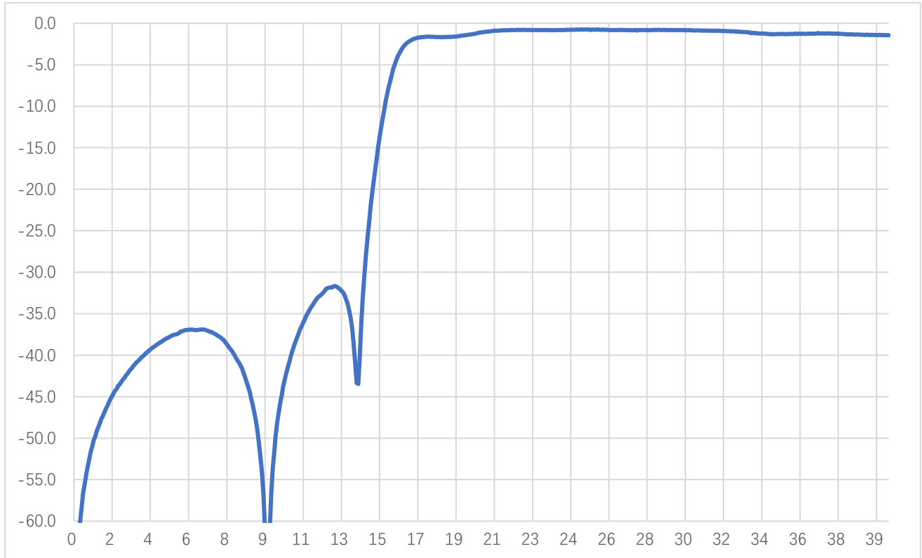
S21 vs Frequency
