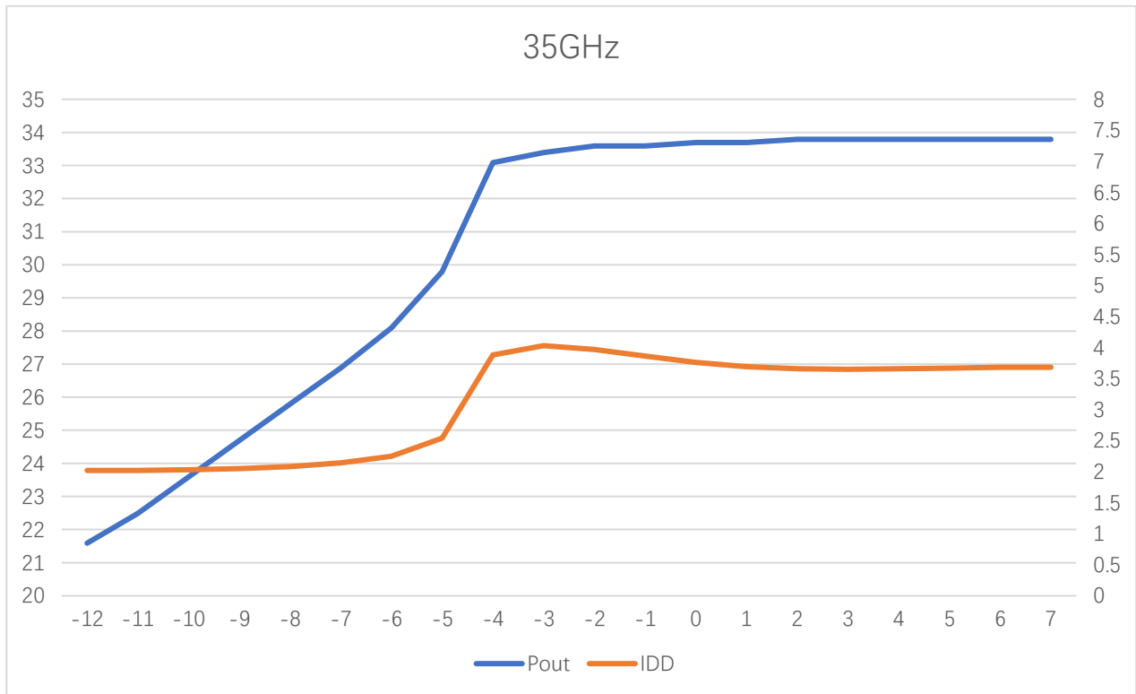
Pout and IDD vs Pin at 35GHz
