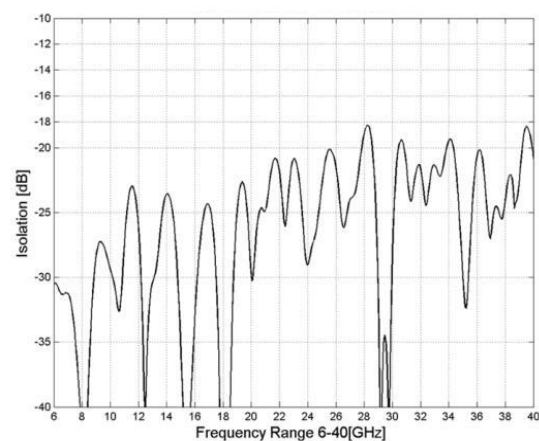
Figure 6: 0-180 Degree Isolation
