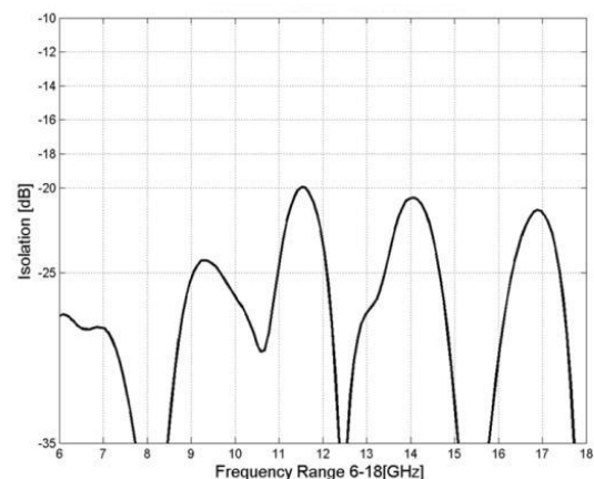
Figure 6: 0-180 Degree Isolation
