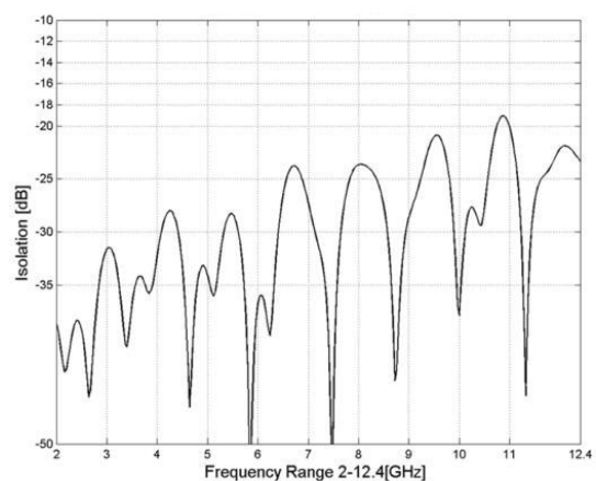
Figure 6: 0-180 Degree Isolation
