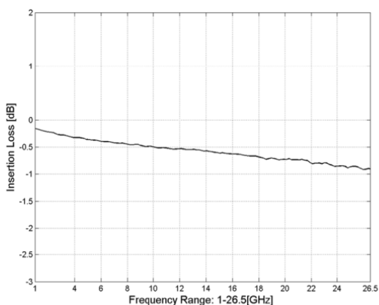
Figure 4: Main Line Insertion Loss
