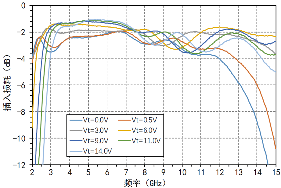
Insertion Loss vs Frequency from 0.5-14V
