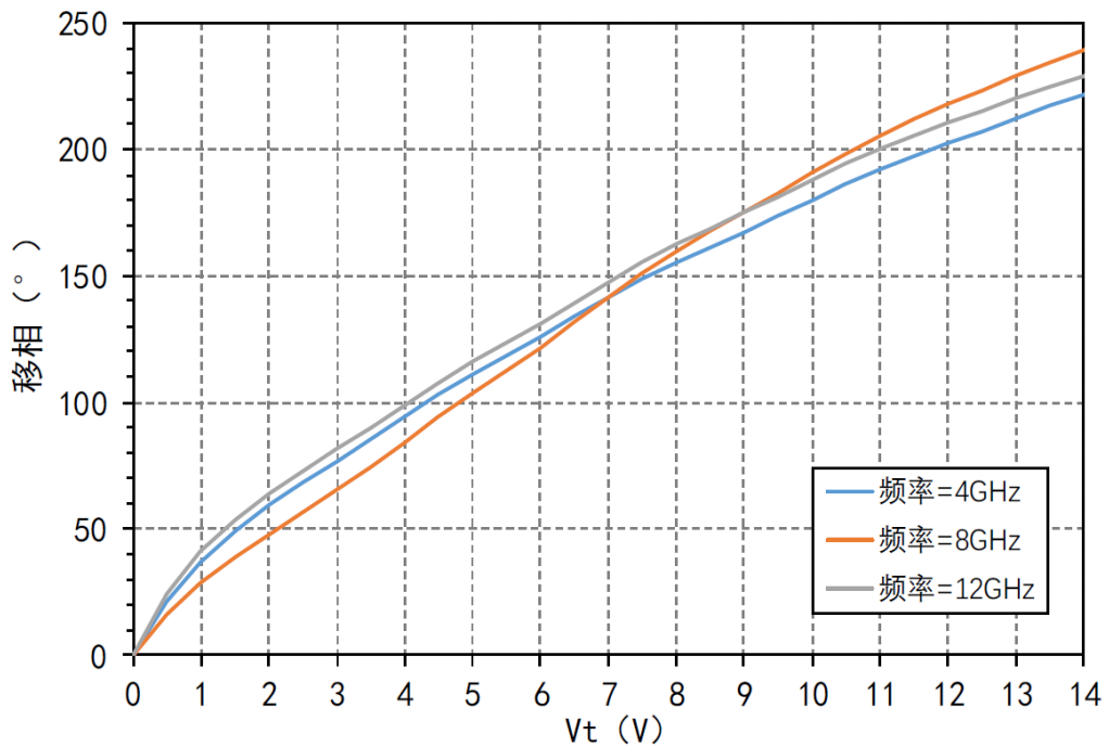
Phase shift vs V_t from 4-12GHz
