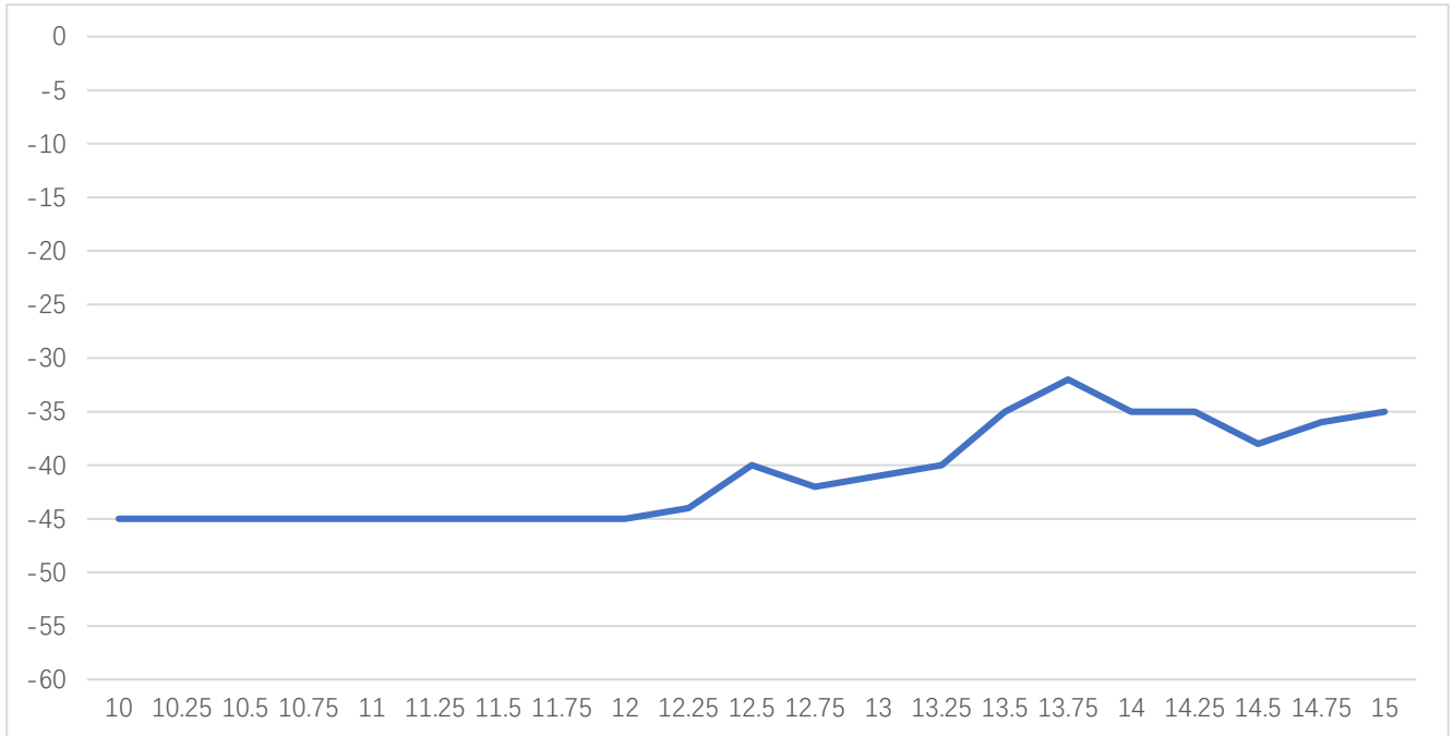
X3 Suppression vs Input frequency, comparing with X4 Pout
