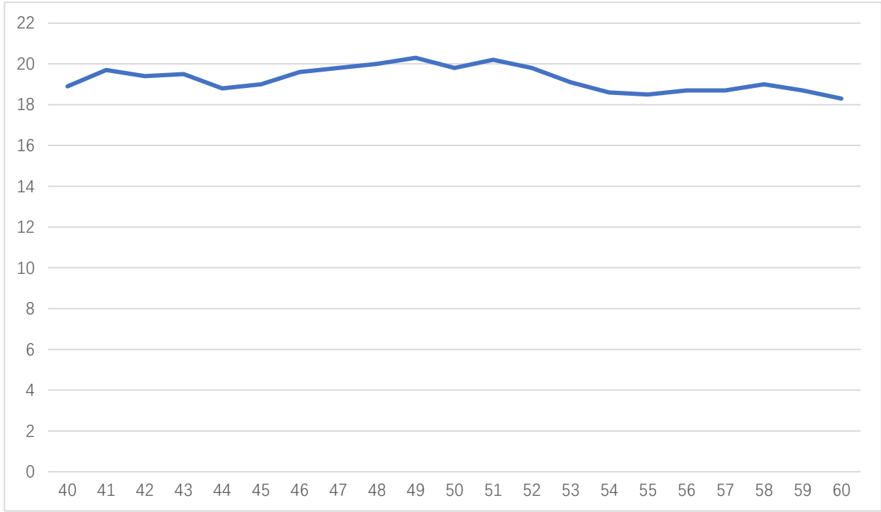
Pout Vs Frequency at Pin=+10dBm
